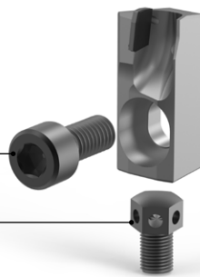
PowerBlue milling cartridge (PBC)
