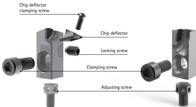
Power milling cartridge (PMC)
