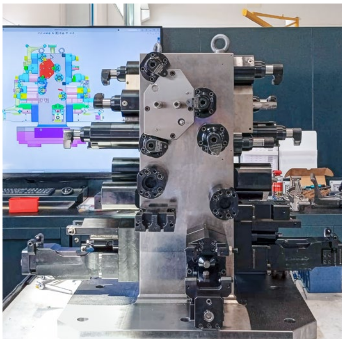
Clamping fixtures are tailored from the outset to the tool design as well as the machining environment and process.
