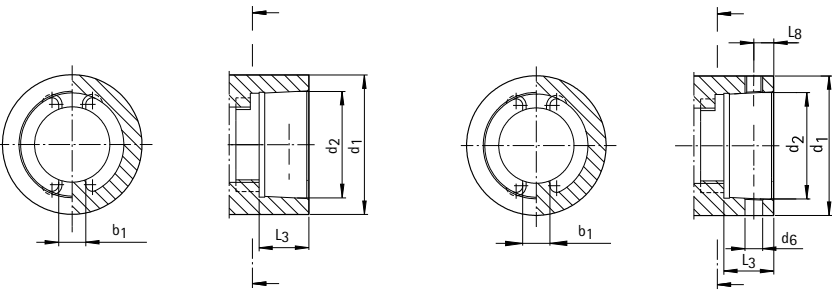
HSK-A for automatic tool change
