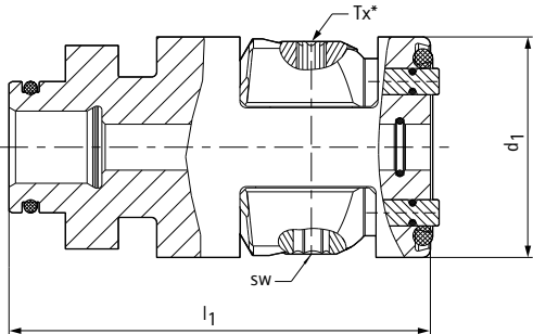
KS clamping cartridges with outer O-ring – version MQL1 for HSK-A and HSK-C
