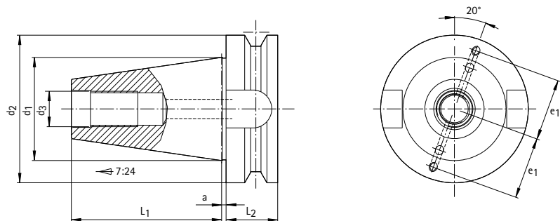
For automatic tool change Form J, Form JF, Form JD and design with data carrier
