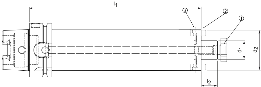
For milling cutter arbors with enlarged face connection diameter according to DIN 69882-3
